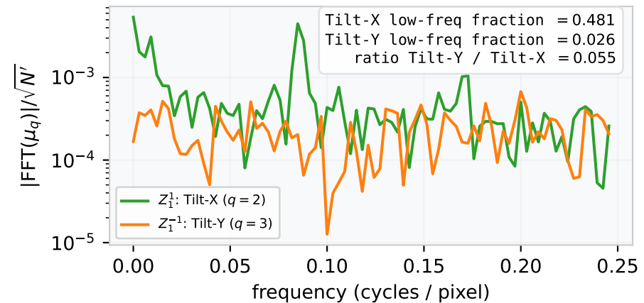
Tilt-X vs Tilt-Y spectra (Tilt-Y diagnostic, m1 minor)
