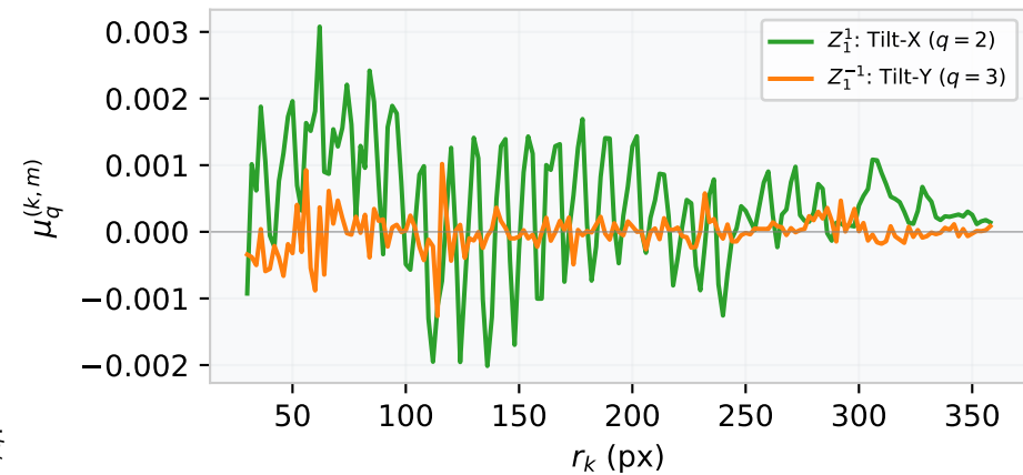
Tilt-X vs Tilt-Y radial profile (ray m = 45 )
